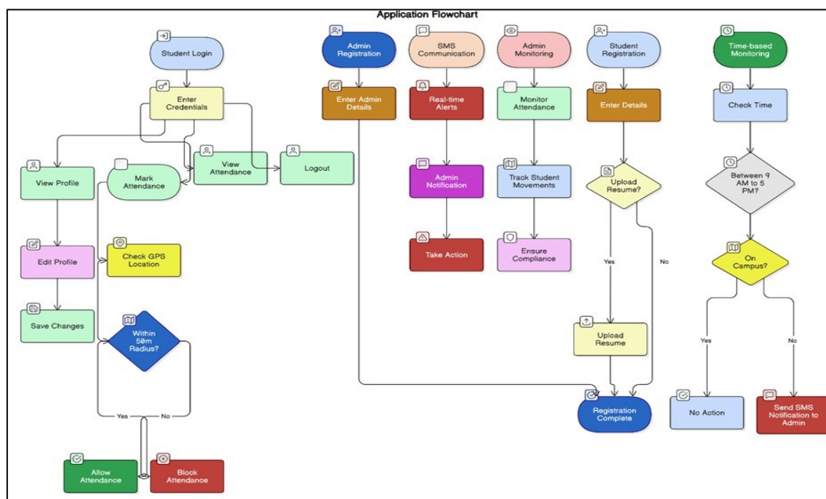
Figure 1: Application Flowchart
